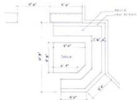
BUILT-IN BENCH / TABLE LAYOUT SCALE: 1/4" = 1'-0"
